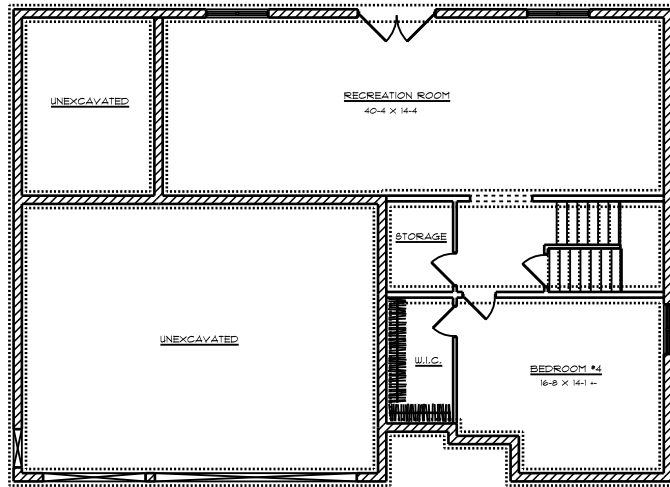
BASEMENT PLAN
